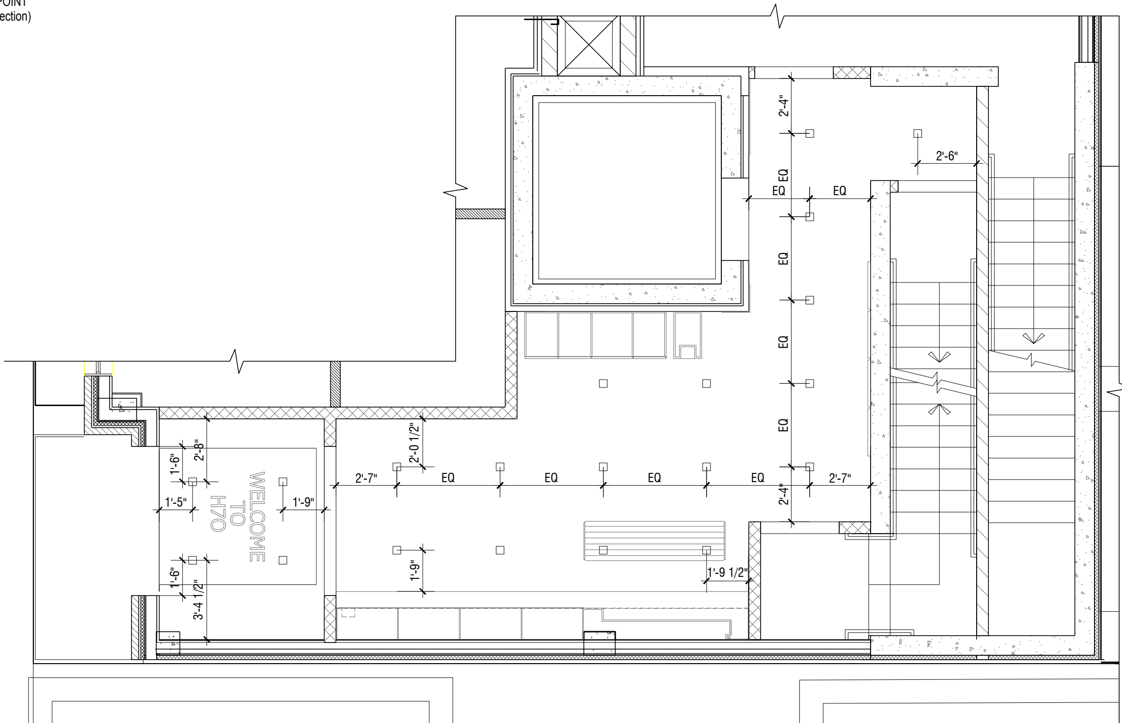
01 REFLECTED CEILING PLAN ID-2
