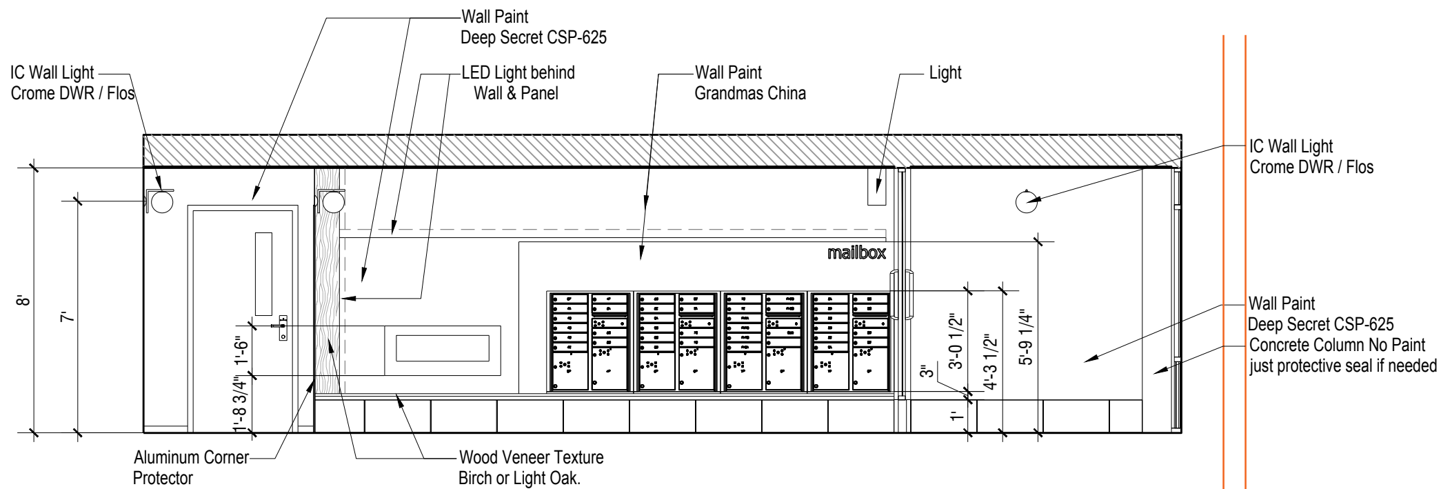
03 INTERIOR ELEVATION ID-3
