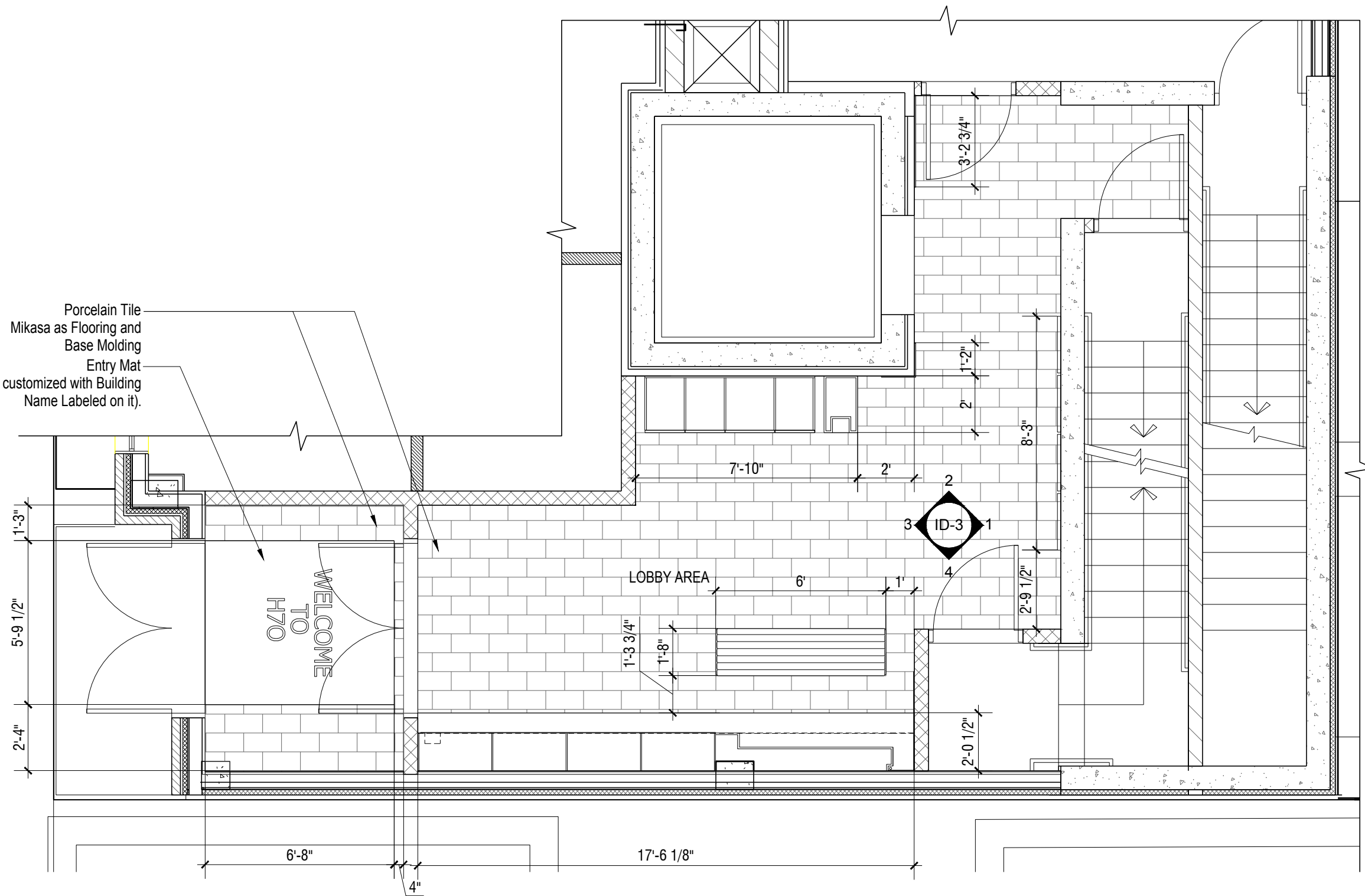
01 FLOOR PLAN ID-1
