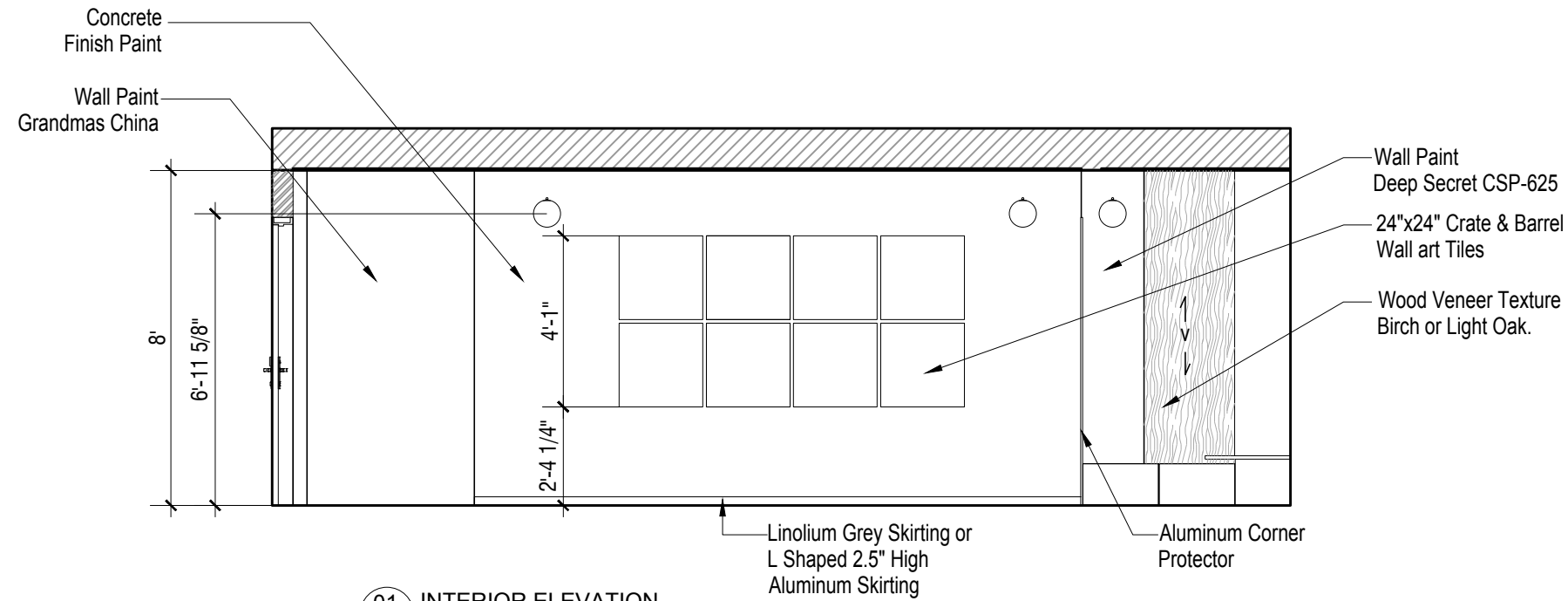
01 INTERIOR ELEVATION
